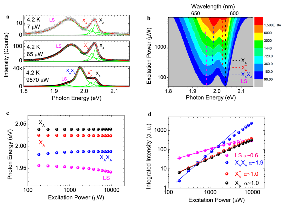
Figure 3. Exciton, trion and biexciton states in a CVD-grown 1L WS 2 at 4.2 K. (a) Photoluminescence spectra at various excitation powers. The total fit curve and subpeaks are shown in red and green, respectively. (b) Photoluminescence intensity mapping versus excitation power and photon energy, where dash curves are guide lines to indicate the spectral evolution. (c) Photon energies of four emission components versus excitation power. (d) Log–log plots of integrated intensities of four emission components versus excitation power. Solid lines are the linear fit curves, and the corresponding \alpha values are the slopes.
